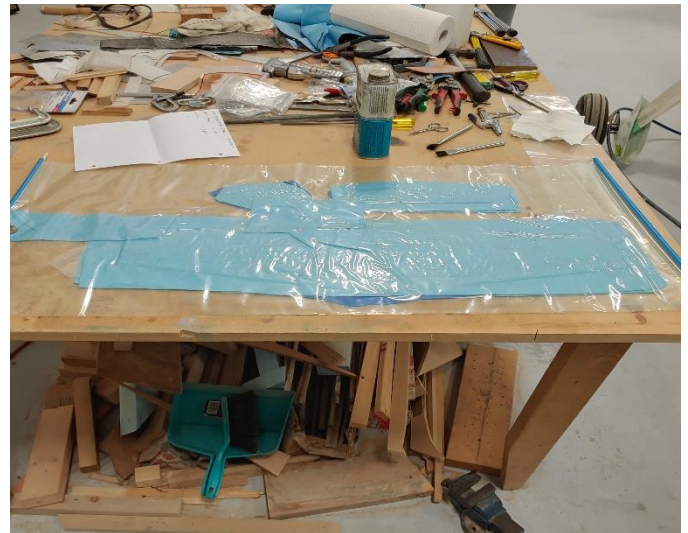
Getting ready for the Vacuum bagging Process.
